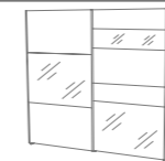
WARDROBE 2 SLIDING DOORS 270 x 250 x 60 cm 31,4" x 74,9" H 54,3"
